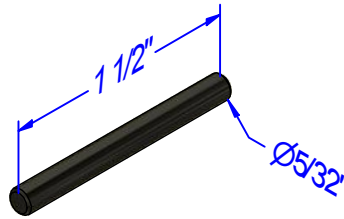
#PC6-120-TW-15 Wheel Axle (1x)
